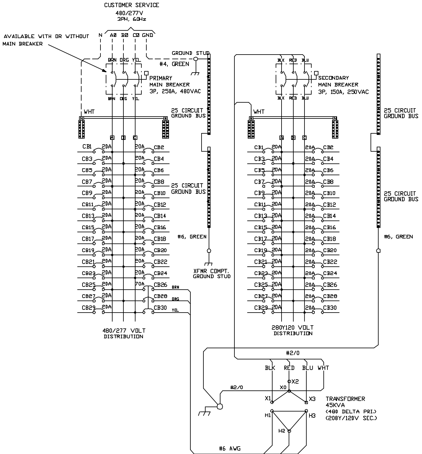
DUAL VOLTAGE UNITIZED DISTRIBUTION SUBSTATION WIRING DIAGRAM WITH NF AND NQOD PANELBOARDS
